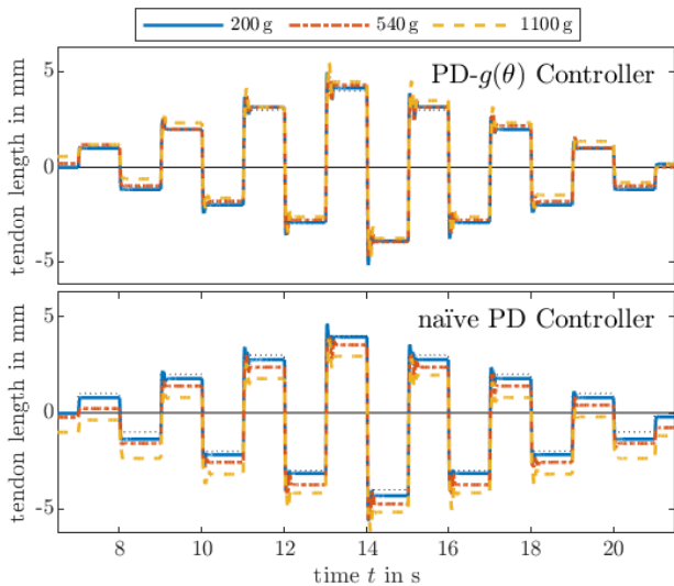
Fig. 4: Comparison of PD controllers with and without gravity compensation. Step responses of different heights with different tendon tensions show that the PD-g(\theta) controller successfully compensates the known load, while the steady-state errors of a naïve PD controller are relative to the load.
