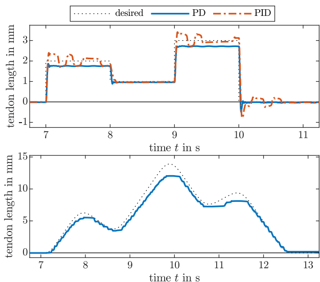
Fig. 6: An actuated flexible beam response to step inputs and a desired C^4 smooth trajectory. The flexible beam induces a variable tendon tension appearing as a variable steady-state and trajectory tracking error. The error correlates with the amount of bending.
