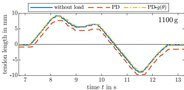
Fig. 5: Following a desired C^4 smooth trajectory with and without load and gravity compensation. The uncompensated load appears as a constant offset in the error. The performance of the PD-g(\theta) controller with load coincides with the performance of the PD controller without load. Note that, in an unloaded case, both controllers behave similarly.
